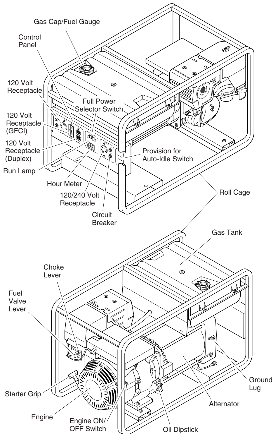
Figure 1 - Portable Generator (Model MGH4000C Shown)
